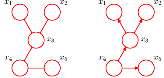
Figure 5 The graph on the left is an undirected tree. If we pick x_4 to be the root node and direct all the edges in the graph to point from the root to the leaf nodes ( x_1 , x_2 and x_5 ), we obtain the directed tree shown on the right.
